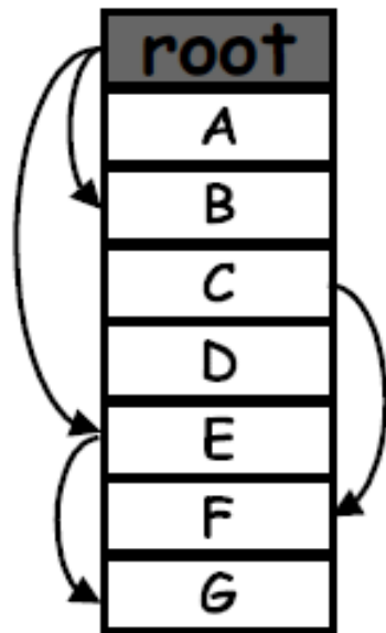
Before GC
