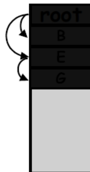
After Compact
