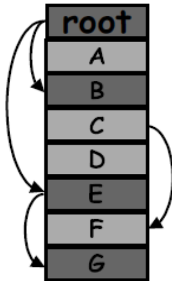
After Mark
