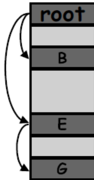
After Sweep
